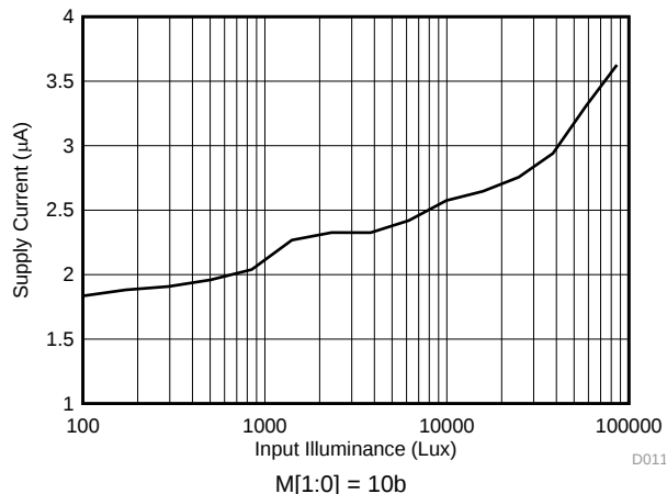
Figure 16. Supply Current vs Input Illuminance
