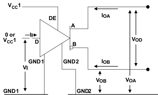
Figure 9. Open Circuit Voltage Test Circuit
