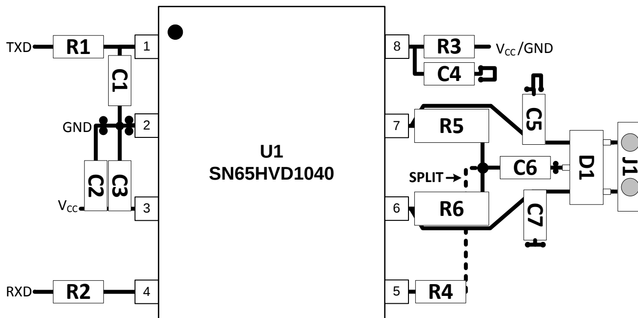
Figure 34. Layout Recommendation
